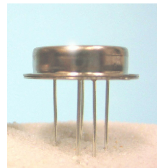
HC 37/U LOW PROFILE
