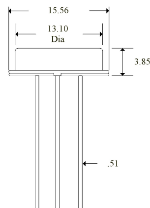
HC 37/U LOW PROFILE
